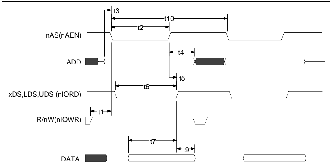
FIGURE 29 - 68000 READ TIMING
